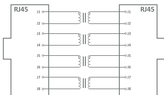
Network isolator MI 1005
