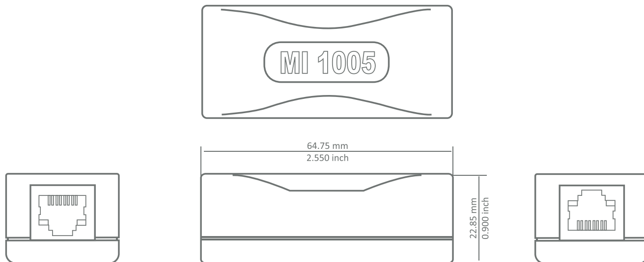
Network isolator MI 1005
